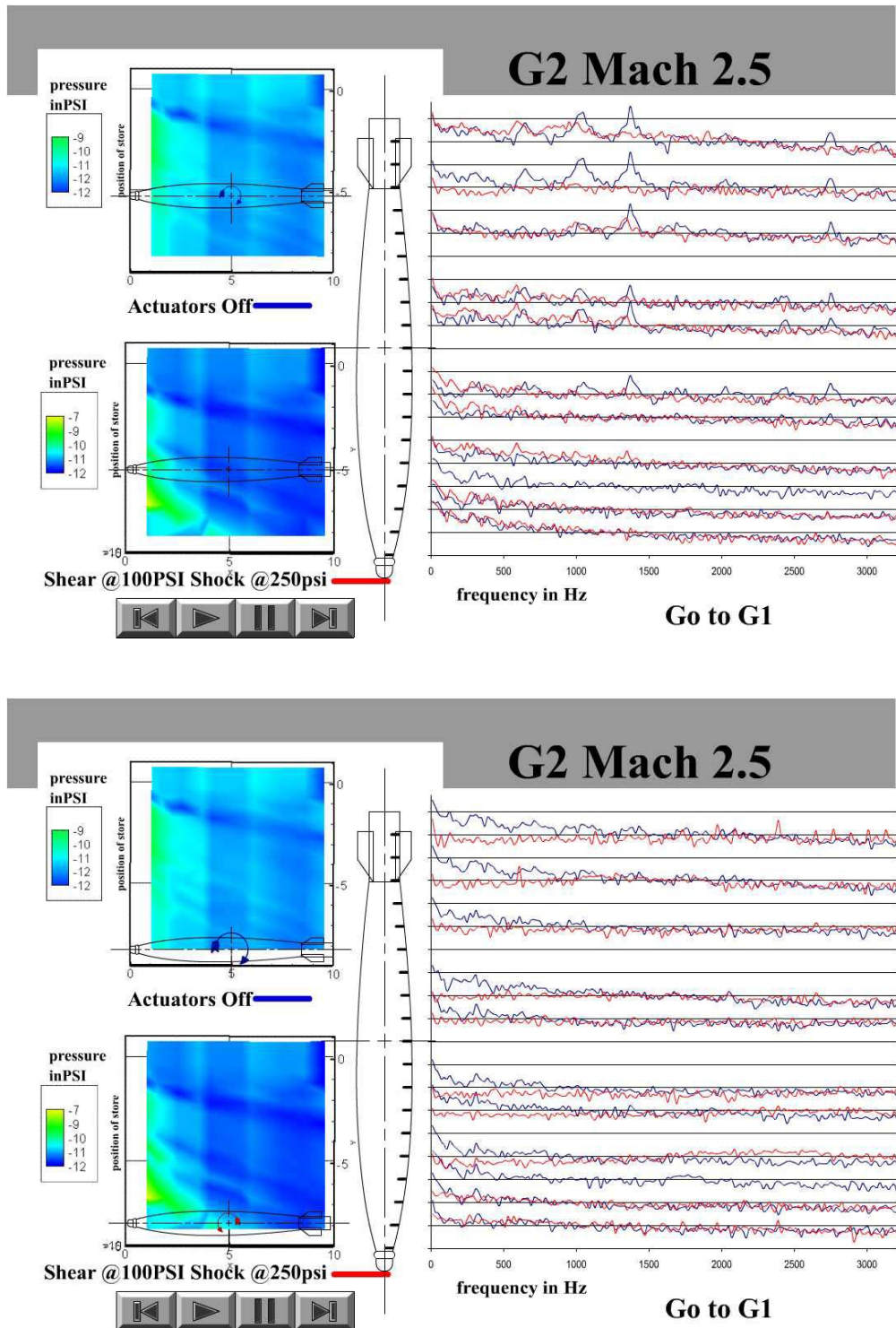
Figure 11: Dynamic pressures recorded on weapon model in mid-bay grid survey (top: weapon in initial grid position; bottom: weapon at grid position before encountering actuator-generated shock)
