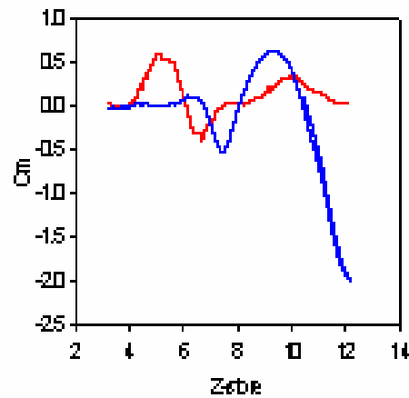
Figure 10: Pitching moment vs. weapon location for mid-bay position at Mach 2.5 (MJ, PRT, and JS actuators)
