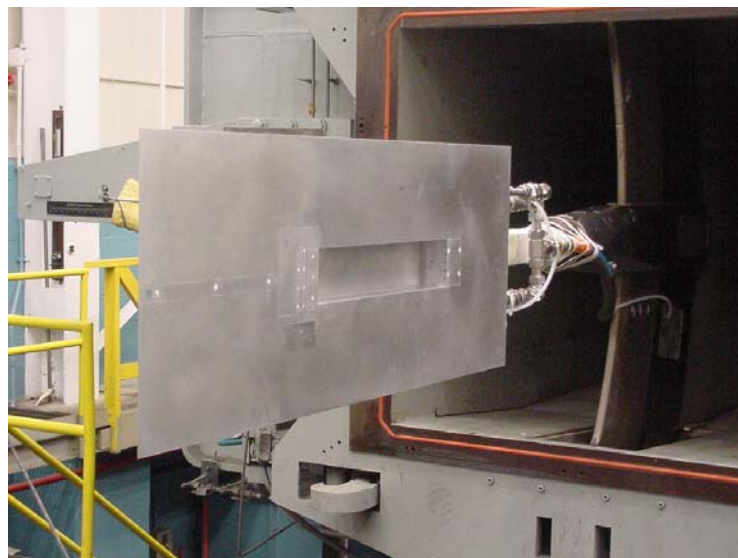
Figure 2: Powered resonance tube bank located upstream of the HIFEX weapons bay
