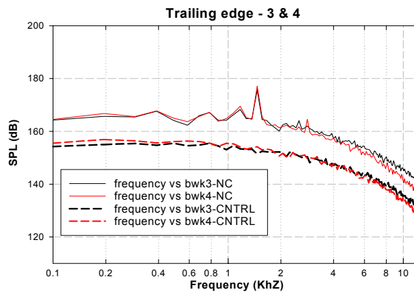
Figure 5: Effect of powered resonance tubes (PRT1) on sound pressure levels in the HIFEX weapons bay (Mach 2.5)
