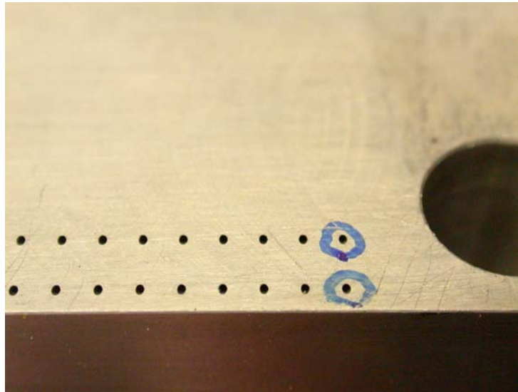
Figure 3: Jet screen slot (0.030 inch x 4 inches) located upstream of the HIFEX weapons bay
