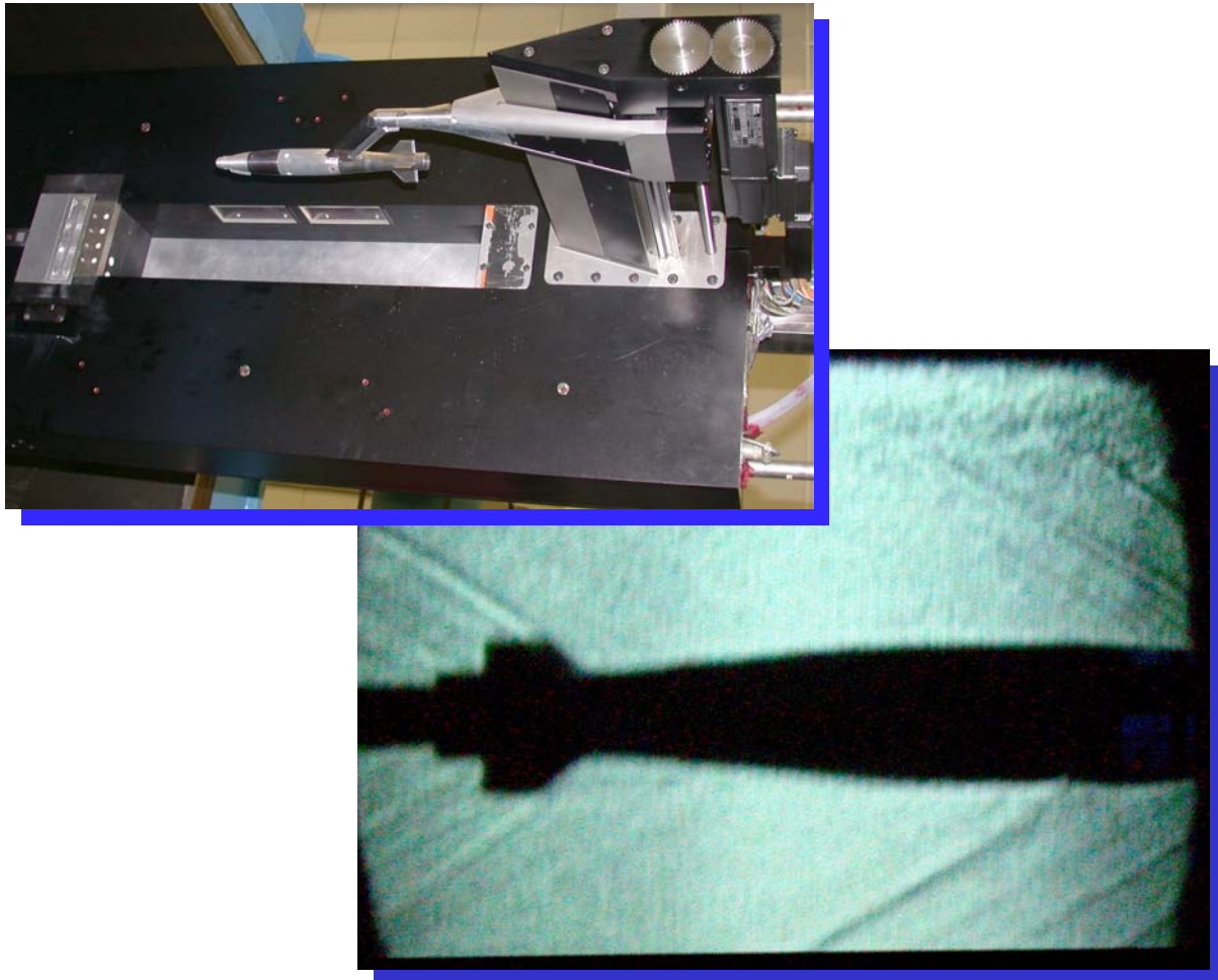
Figure 9: Arrangement of HIFEX weapons bay and MK-82 JDAM models for grid testing in the Boeing Polysonic Wind Tunnel
