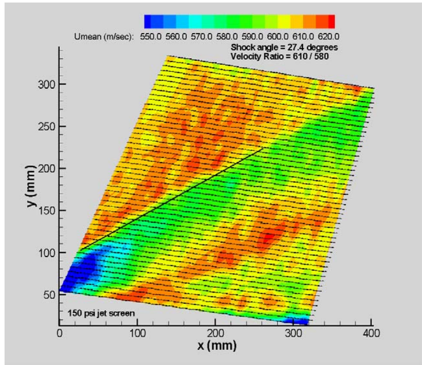
Figure 8: Velocity field in vicinity of HIFEX weapons bay with jet screen operating at 150 psig (Mach 2.5)
