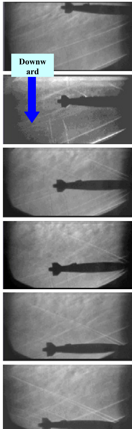
Figure 12: Sequence of high-speed video images for controlled release of MK-82 JDAM model from the mid-bay position at Mach 3.2
