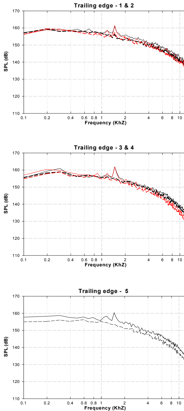
Figure 7: Effect of Microjets (MJ1, 100 psig supply pressure) on sound pressure levels in the HIFEX weapons bay (Mach 3.2)
