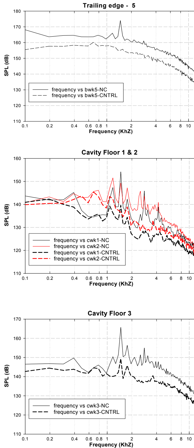
Figure 6: Effect of Microjets (MJ1, 100 psig supply pressure) on sound pressure levels in the HIFEX weapons bay (Mach 2.5).
